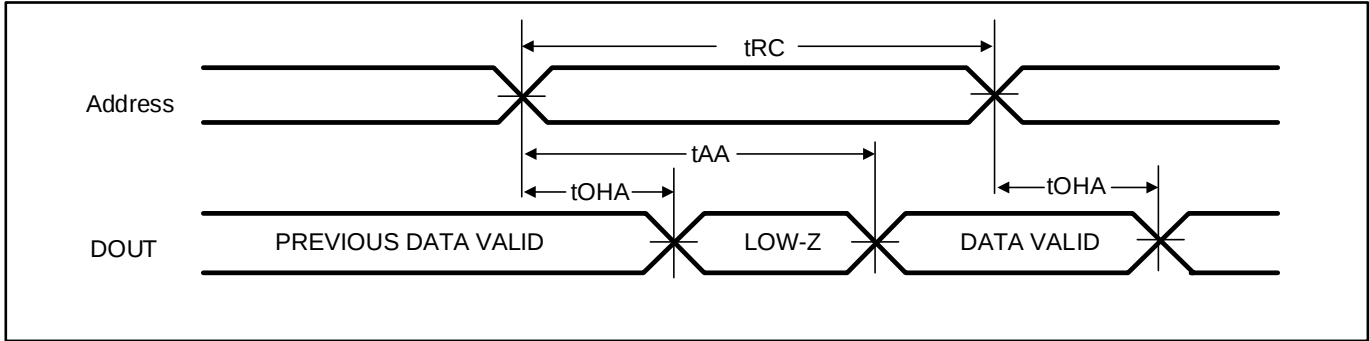
READ CYCLE NO. 1 (1) (ADDRESS CONTROLLED) (CS1# = OE# = LOW, CS2 = WE# = HIGH)
