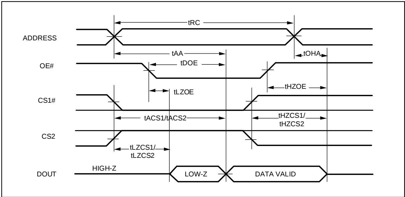
READ CYCLE NO. 2 (1) (OE# CONTROLLED)
