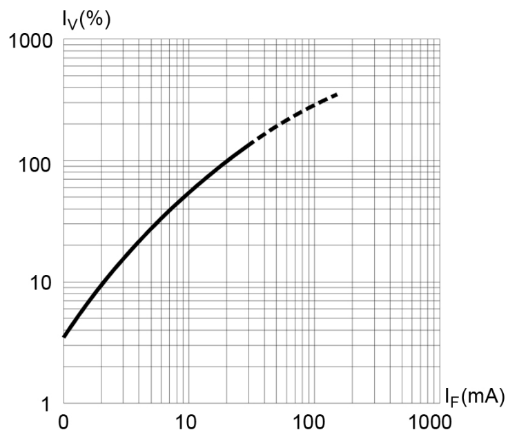
Fig. 3 Relative Luminous Intensity vs. Forward Current
