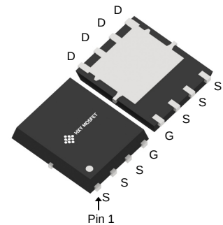
DFN5X6-8L (DFN(5x6))
