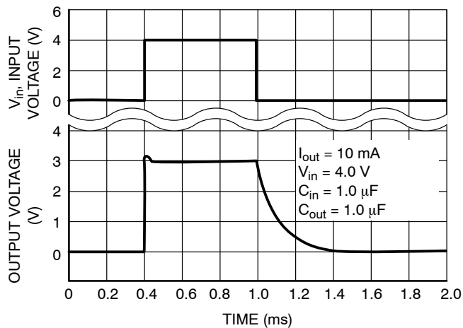
Figure 11. Turn-on Response
