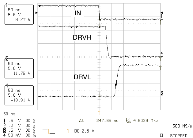
Figure 5. DRVH Fall and DRVL Rise Times
