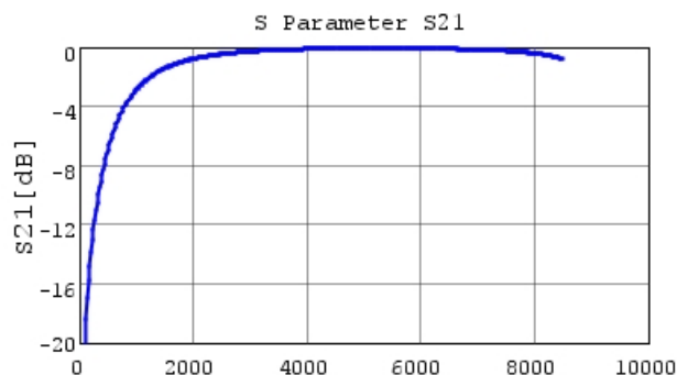
GRM1885C2A1R6CA01 S21 DCOV, 25degC
