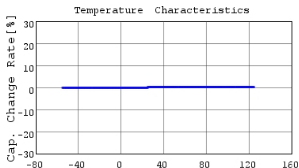
GRM1885C2A1R6CA01 C-Temp. capchange, DCOV, 1
