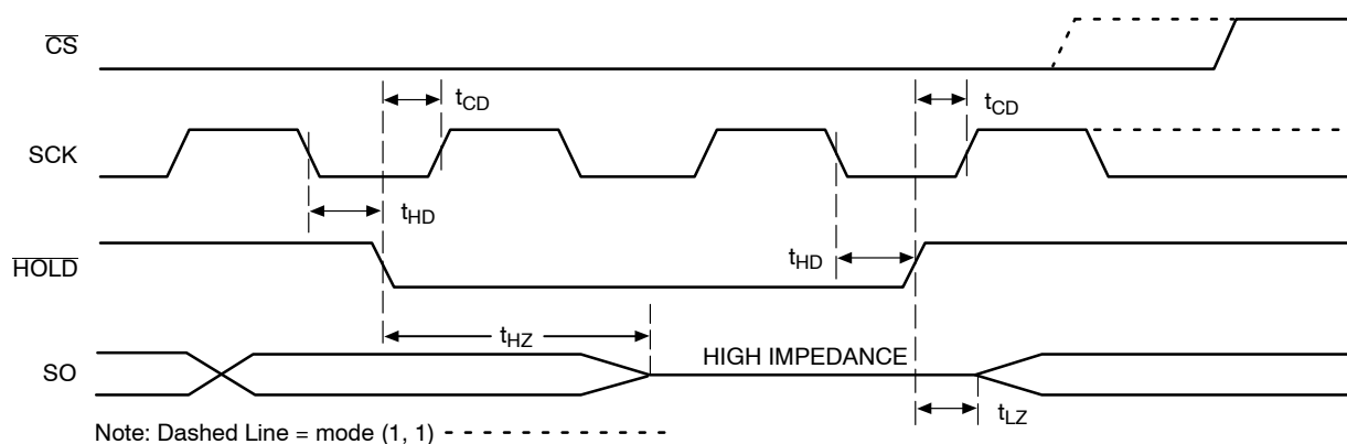
Figure 11. HOLD Timing
