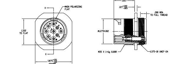
Part Dimensions for ATC-09-9-1939PN
