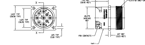
Part Dimensions for ATC-10-9-1939PN
