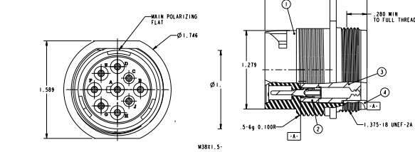
Part Dimensions for ATC-10-9-1939PN
