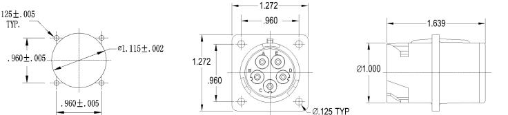
Part Dimensions for ATC-11-9-1939PN
