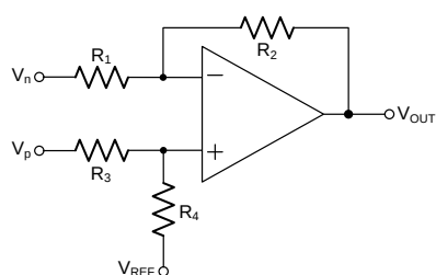
Figure 5. Differential Amplifier
