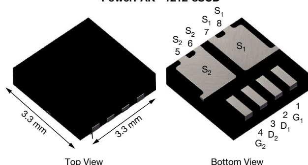
PowerPAK® 1212-8SCD
