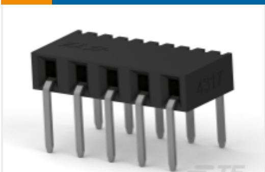
TE Part #2307706-5 5P,2MM,B-B,REC,SRHZ,2.1,0.38AU,TR
