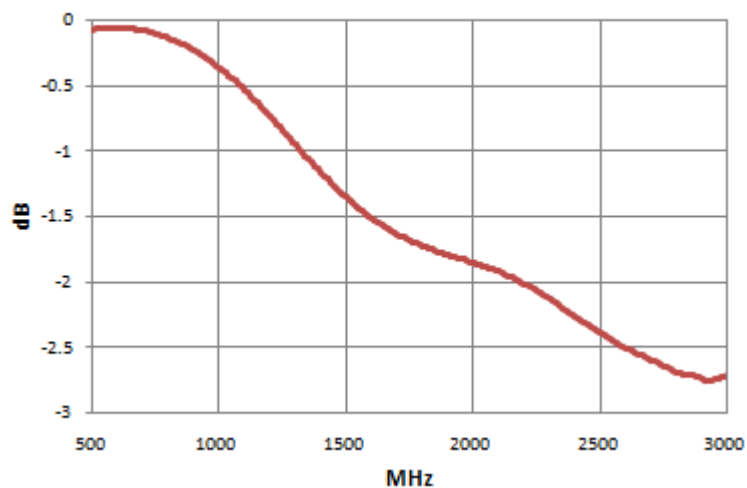
Insertion Loss
