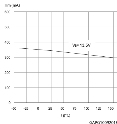
Figure 8. Current limitation vs. T_j
