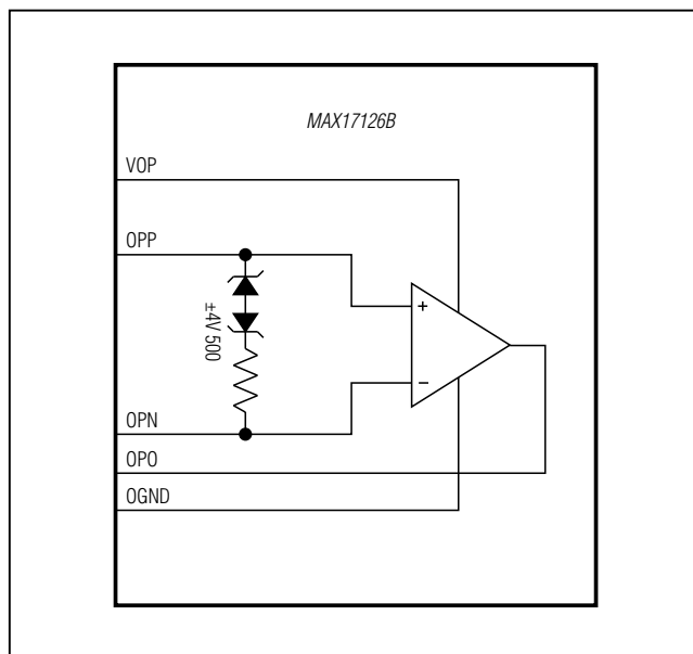
Figure 6. Op Amp Input Clamp Structure
