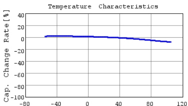
■ GRT033C80J332KE01 C-Temp. capchange, DC0.0V,
