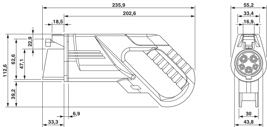
Dimensional drawing
