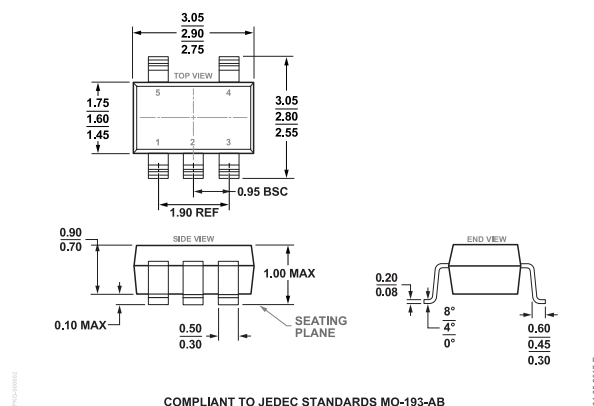
Figure 63. 5-Lead Thin Small Outline Transistor Package [TSOT] (UJ-5) Dimensions shown in millimeters
