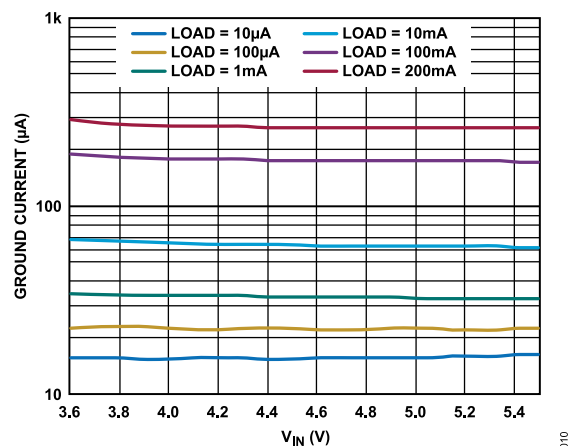
Figure 12. Ground Current ( I_{GND} ) vs. Input Voltage ( V_{IN} )
