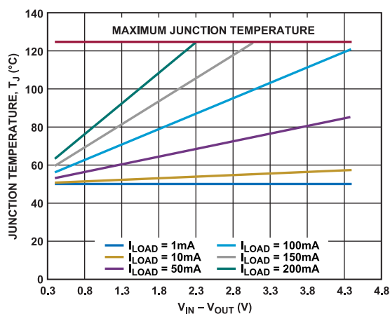
Figure 55. LFCSP 100 mm 2 of PCB Copper, T_A = 50^\circ\text{C}
