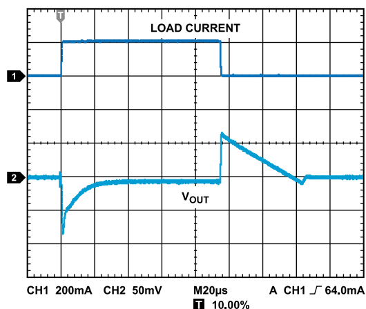
Figure 24. Load Transient Response, C_{IN} = C_{OUT} = 1\text{ μF} , I_{LOAD} = 1\text{ mA to } 200\text{ mA}
