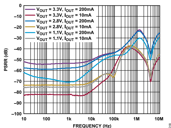
Figure 20. Power Supply Rejection Ratio (PSRR) vs. Frequency at Various Output Voltages and Load Currents, V_{OUT} - V_{IN} = 0.5\text{ V} , Except for V_{OUT} = 1.1\text{ V} , V_{IN} = 2.2\text{ V}
