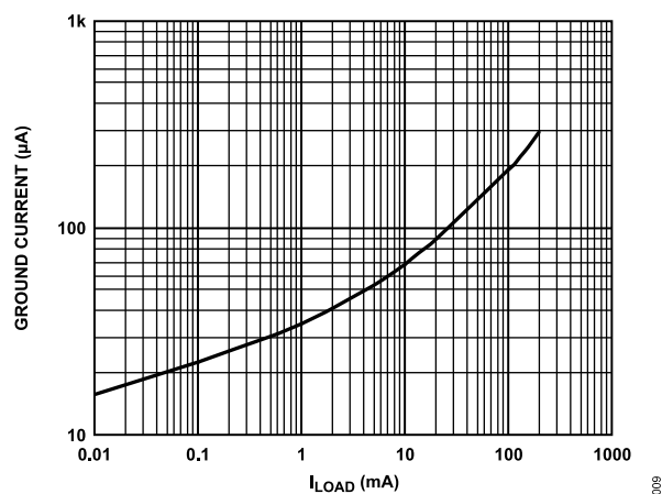
Figure 11. Ground Current ( I_{GND} ) vs. Load Current ( I_{LOAD} )
