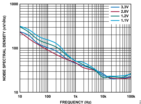
Figure 23. Output Noise Spectral Density vs. Frequency, V_{IN} = 5\text{ V} , I_{LOAD} = 10\text{ mA} , C_{OUT} = 1\text{ μF}
