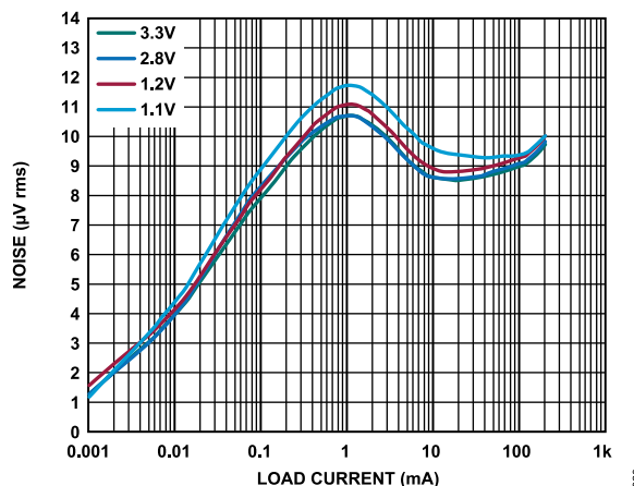
Figure 22. Output Noise vs. Load Current for Various Output Voltages, V_{IN} = 5\text{ V} , C_{OUT} = 1\text{ μF}
