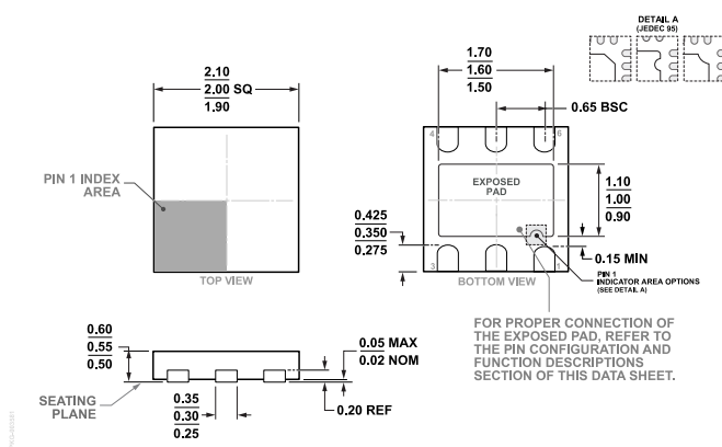
Figure 65. 6-Lead Lead Frame Chip Scale Package [LFCSP] 2.00 mm x 2.00 mm Body and 0.55 mm Package Height (CP-6-3) Dimensions shown in millimeters
