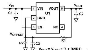
Figure 33. Adjustable LDO Using the ADP151
