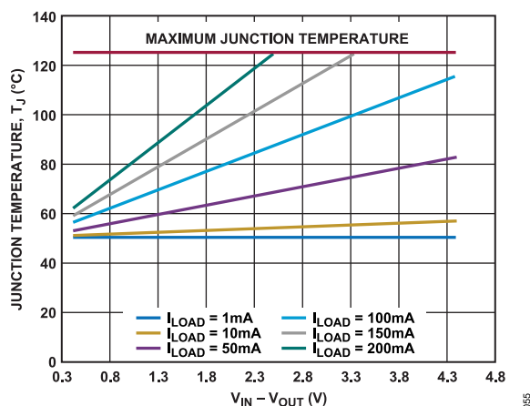
Figure 54. LFCSP 500 mm 2 of PCB Copper, T_A = 50^\circ\text{C}
