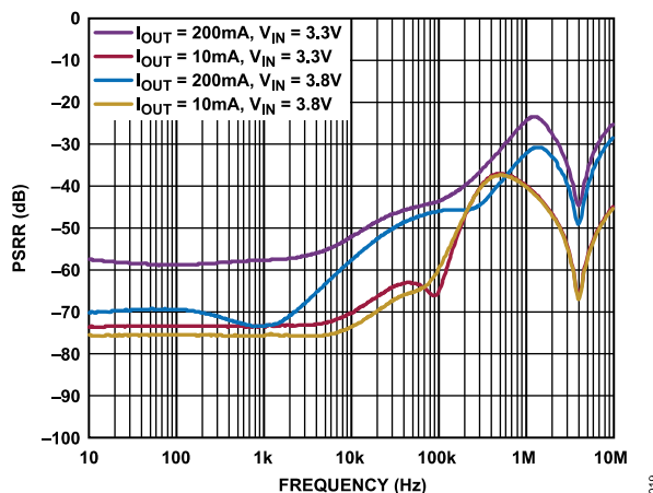
Figure 21. Power Supply Rejection Ratio (PSRR) vs. Frequency at Various Voltages and Load Currents, V_{OUT} = 2.8\text{ V}
