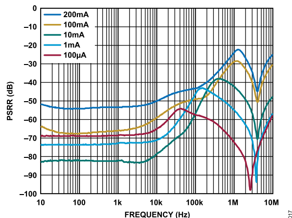
Figure 19. Power Supply Rejection Ratio (PSRR) vs. Frequency, V_{OUT} = 3.3\text{ V} , V_{IN} = 3.8\text{ V}
