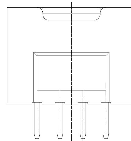
ENGAGEMENT FIGURE (2:1)
