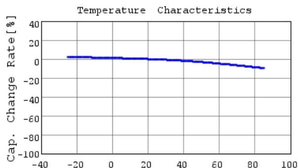
GRM31CB10J475KA01 C-Temp. capchange, DC0.0V,
