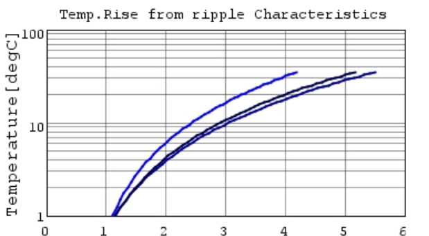
GRM31CB10J475KA01 Temp.rise — 100kHz
