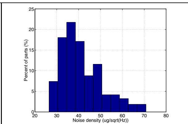
Figure 18. Noise density at 3.3V (z axis)
