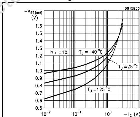
Figure 5. Base-emitter saturation voltage
