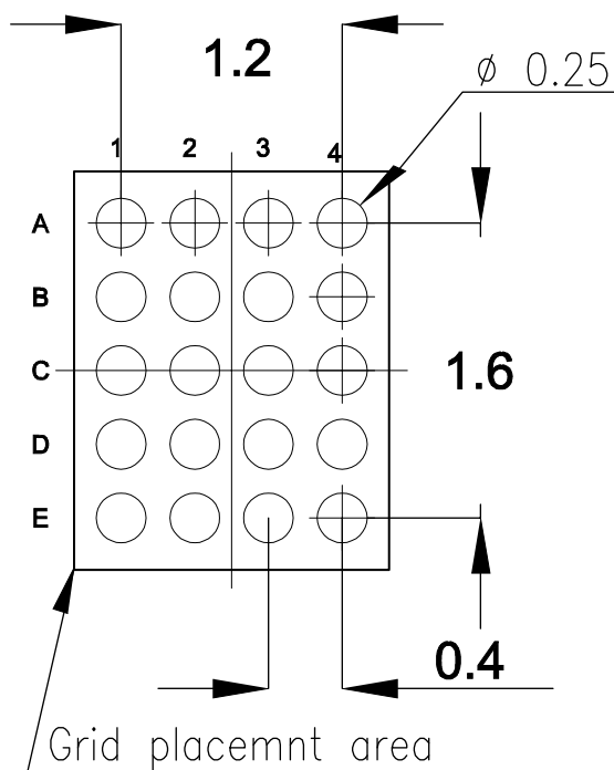
Figure 26. Flip-Chip 20 (1.71 x 2.16 x 0.5 mm) recommended footprint
