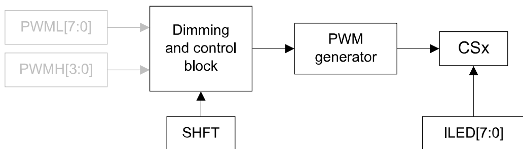
Figure 5. Analog dimming
