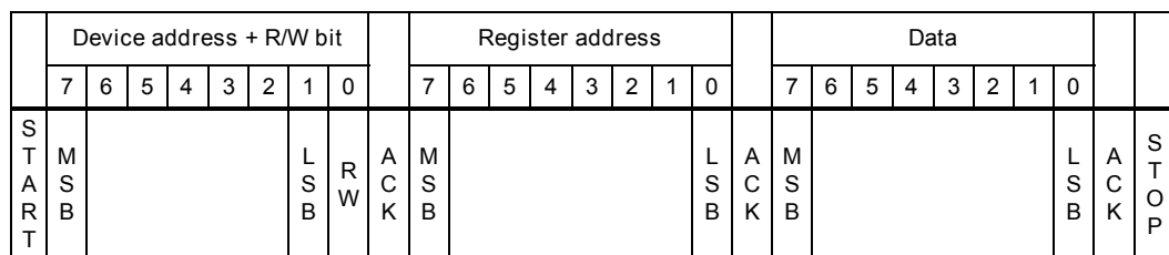
Figure 15. Interface protocol
