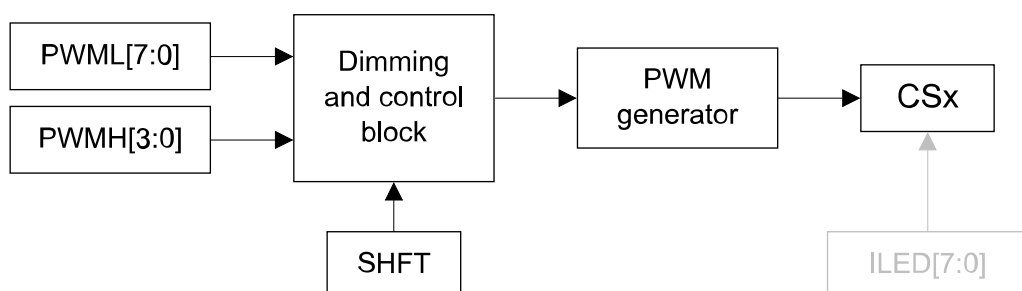
Figure 6. Digital dimming
