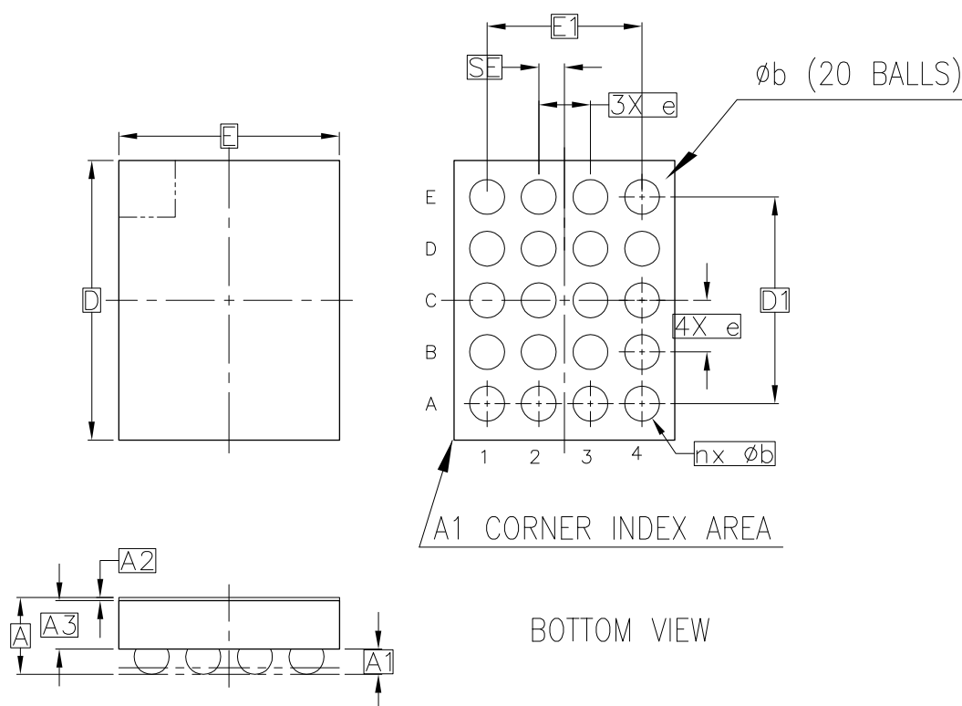
Figure 25. Flip-Chip 20 (1.71 x 2.16 x 0.5 mm) package outline
