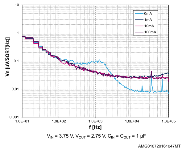
Figure 21: Noise density
