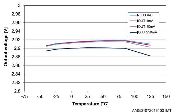
Figure 5: Output voltage vs temperature ( V_{IN} = 5.5\text{ V} )
