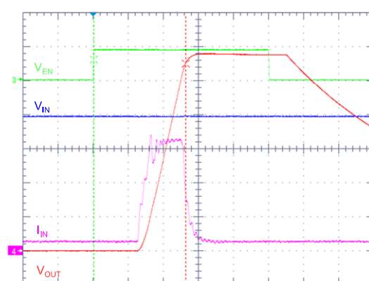
Figure 25: Inrush current
