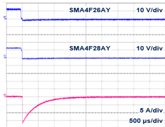
Figure 12. ISO7637-2 pulse 1: V_s = -150 V with 12 V battery
