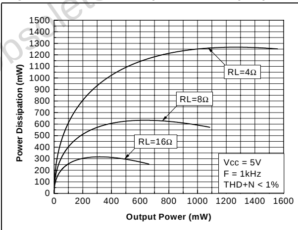
Figure 60. Power dissipation vs. output power
