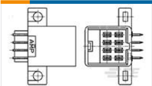
TE Part #172244-1 DLI 8POS CAP ASSY H TIN
