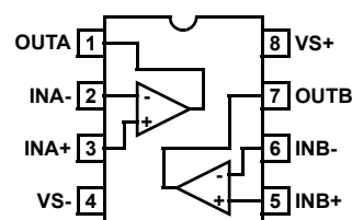
EL5257 (8 LD SOIC) TOP VIEW
