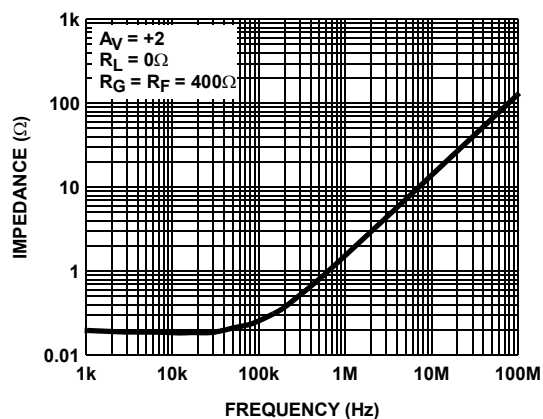
FIGURE 24. OUTPUT IMPEDANCE
