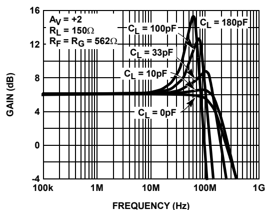
FIGURE 6. SMALL SIGNAL FREQUENCY RESPONSE FOR VARIOUS C_L
