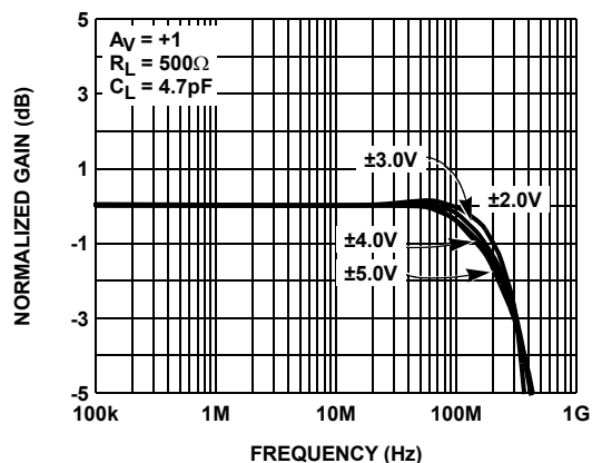
FIGURE 8. FREQUENCY RESPONSE vs POWER SUPPLY
