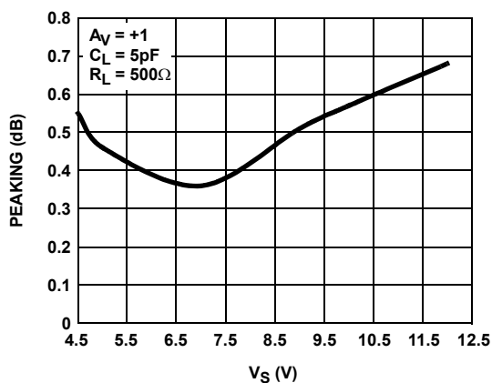
FIGURE 28. PEAKING vs SUPPLY VOLTAGE
