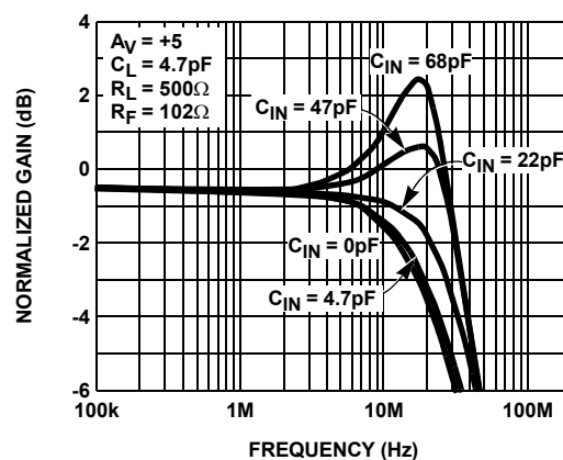
FIGURE 14. SMALL SIGNAL FREQUENCY RESPONSE FOR VARIOUS C_{IN}
