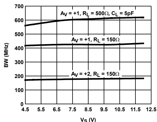
FIGURE 20. BANDWIDTH vs SUPPLY VOLTAGE
