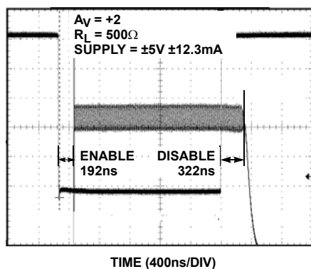
FIGURE 27. ENABLE/DISABLE RESPONSE
