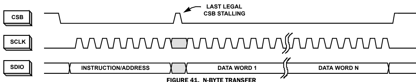
FIGURE 41. N-BYTE TRANSFER
