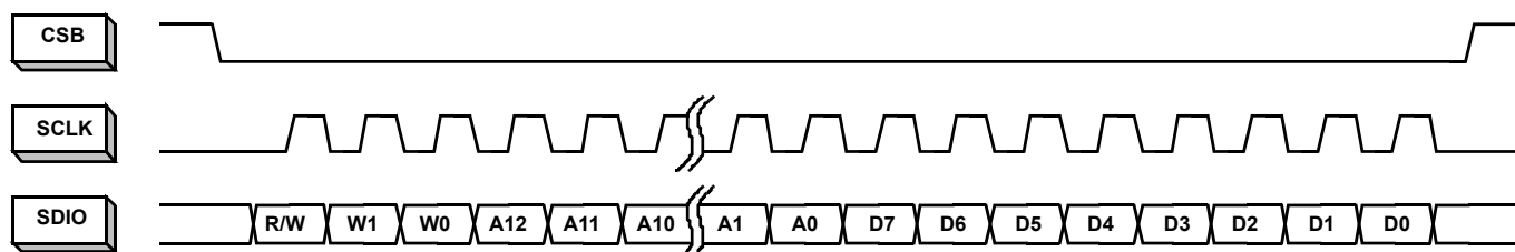
FIGURE 36. MSB-FIRST ADDRESSING
