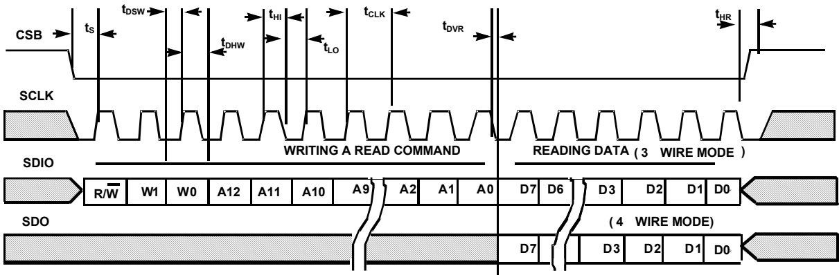
FIGURE 39. SPI READ
