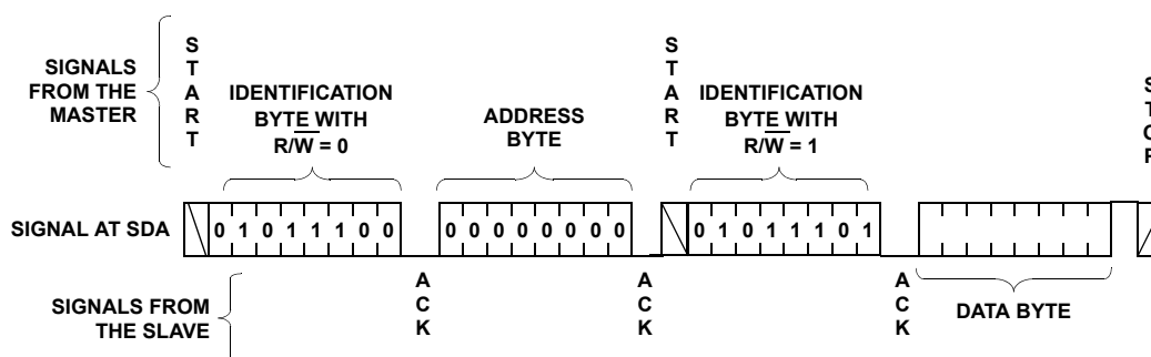
FIGURE 4. READ SEQUENCE
