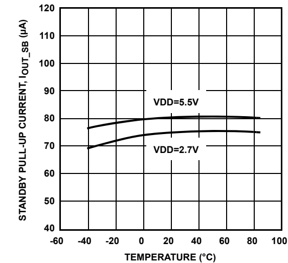
FIGURE 3. STANDBY PULL-UP CURRENT. SMBus1,2=V DD -0.5V
