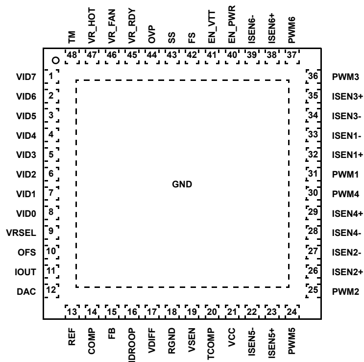
(48 LD QFN) TOP VIEW
