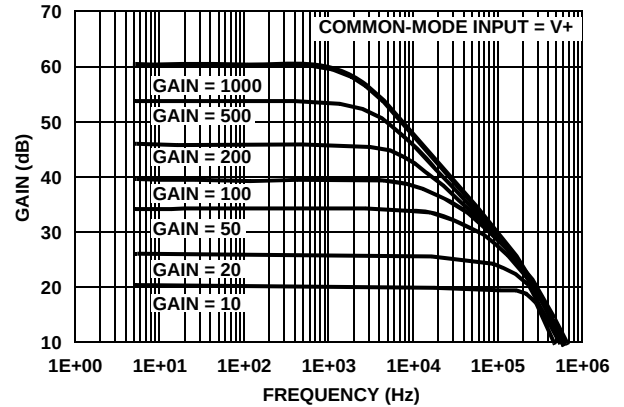
FIGURE 2. ISL28273 FREQUENCY RESPONSE vs CLOSED LOOP GAIN ( V_{CM} = V_+ )
