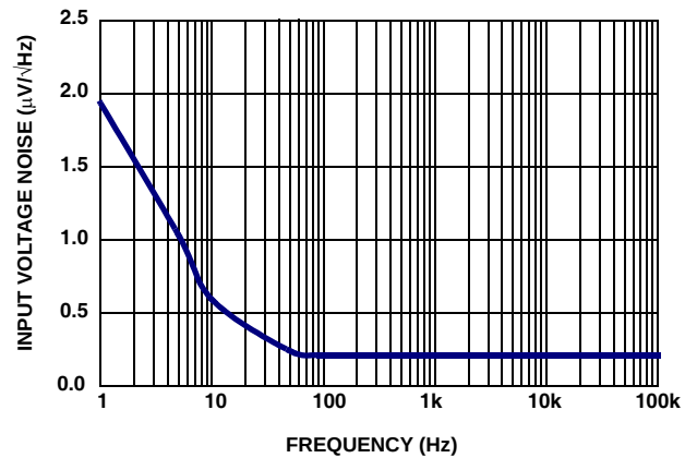
FIGURE 16. ISL28273 INPUT VOLTAGE NOISE SPECTRAL DENSITY (GAIN = 10)
