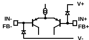
CIRCUIT 1B
