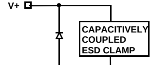
CIRCUIT 4
