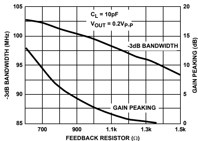
FIGURE 24. BANDWIDTH AND GAIN PEAKING vs FEEDBACK RESISTOR
