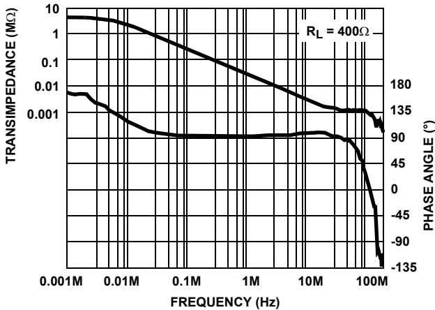
FIGURE 57. TRANSIMPEDANCE vs FREQUENCY
