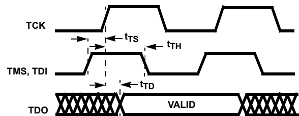
FIGURE 20. JTAG TIMING
