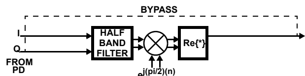
FIGURE 5. IF CONVERTER IN REAL 1X MODE OPERATION
