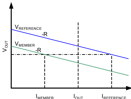
FIGURE 26. ACTIVE CURRENT SHARING
