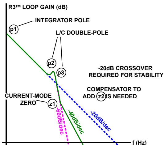
FIGURE 9. UNCOMPENSATED INTEGRATOR OPEN-LOOP RESPONSE
