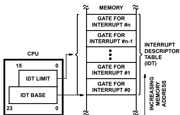
FIGURE 16. INTERRUPT DESCRIPTOR TABLE DEFINITION
