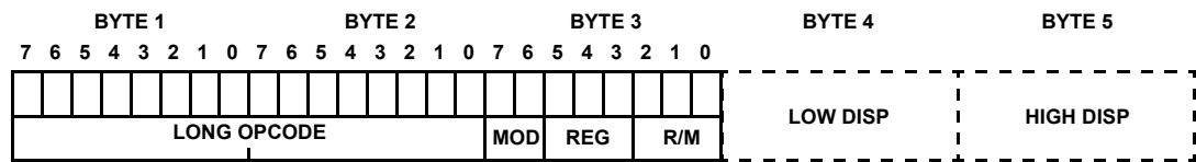
FIGURE 40. 80C286 INSTRUCTION FORMAT EXAMPLES
