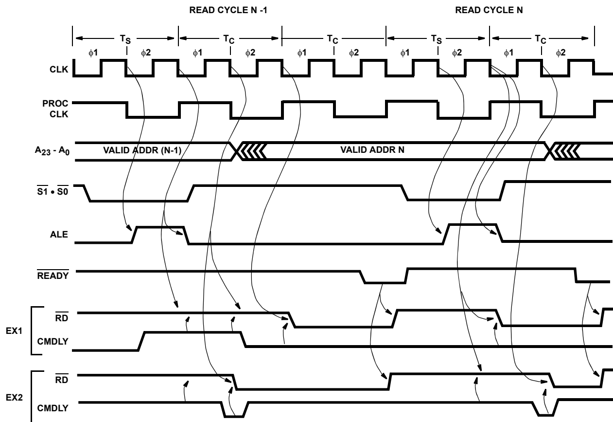
FIGURE 23. CMDLY CONTROLS THE LEADING EDGE OF COMMAND SIGNAL
