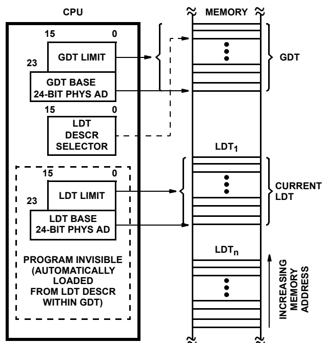
FIGURE 14. LOCAL AND GLOBAL DESCRIPTOR TABLE DEFINITION
