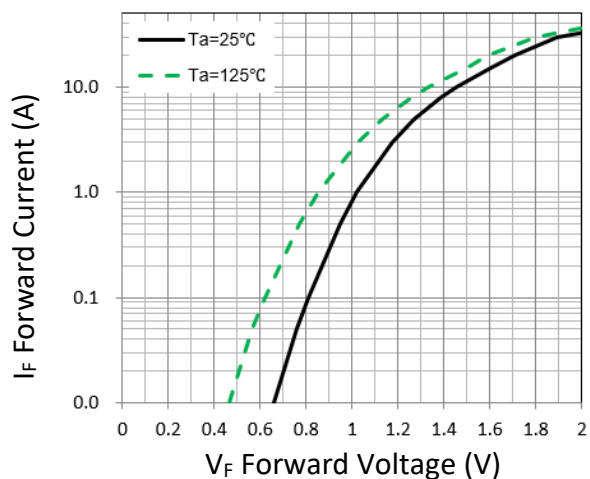
Figure 1. Forward Characteristic(typ.)
