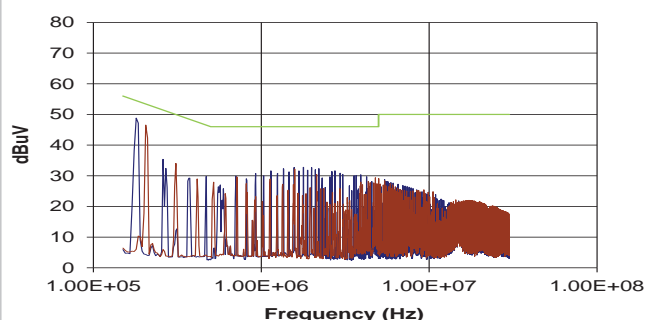
NXF1S0305MC (Average)
