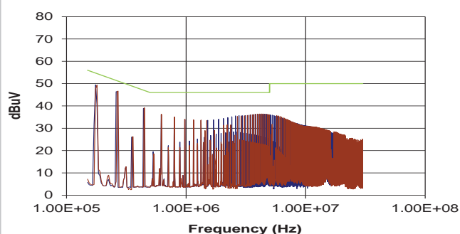
NXF1S0305MC (Average)
