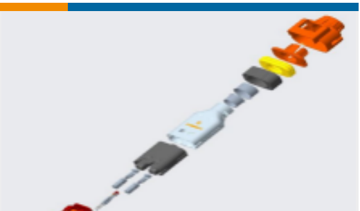
TE Part #YHV280-2PM-P-4MM-B HVA280-2phm,pass,4sqmm,Key B
