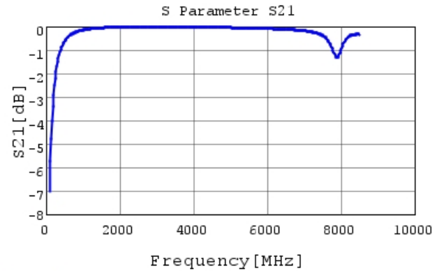
GJM1555C1H7R9BB01 S21 DC0V, 25degC
