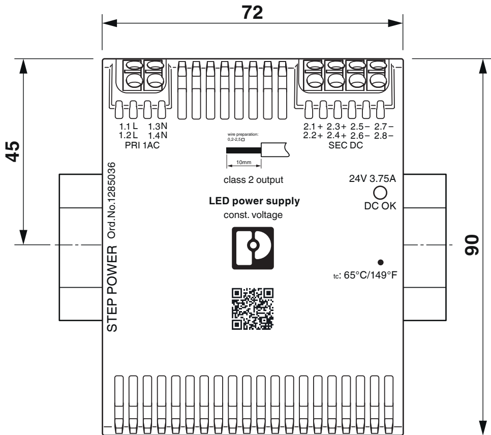
Dimensional drawing
