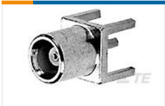
TE Part #829558-4 MCX GE KU LEI
