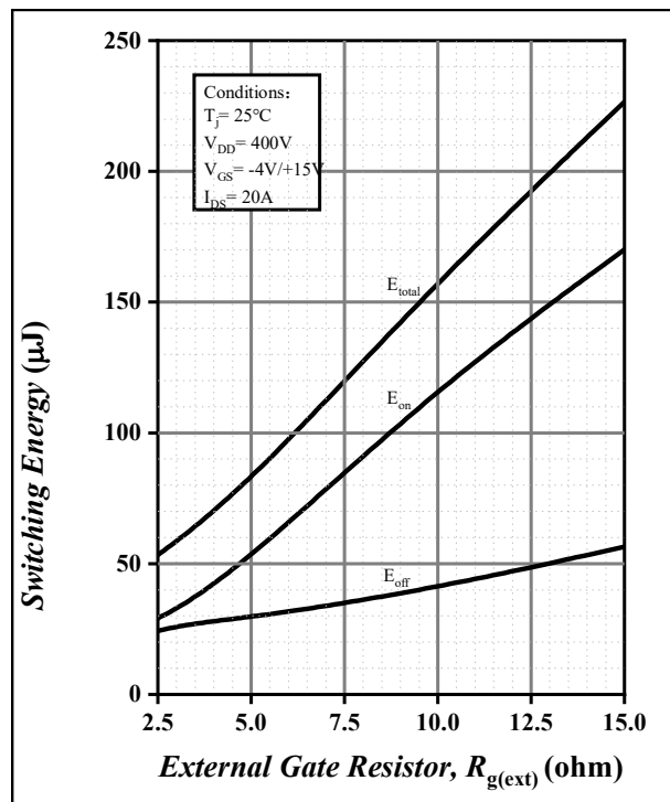
Figure 16. Clamped Inductive Switching Energy vs. R_{g(ext)}
