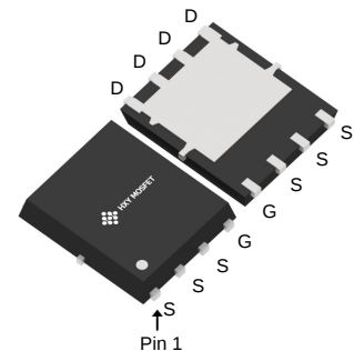
DFN5X6-8L (Power-56-8)
