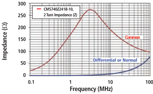
CM5740Z241B-10, 2 Turn Impedance (Z)
