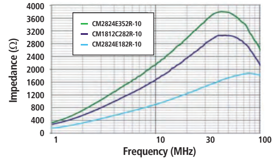
Impedance (Z) versus Frequency
