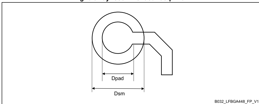
Figure 70. LFBGA - 448 balls, 18x18 mm, 0.8 mm pitch, low profile fine pitch ball grid array recommended footprint
