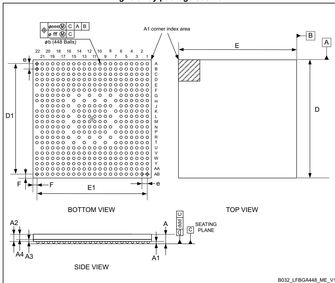
Figure 69. LFBGA - 448 balls, 18x18 mm, 0.8 mm pitch, low profile fine pitch ball grid array package outline
