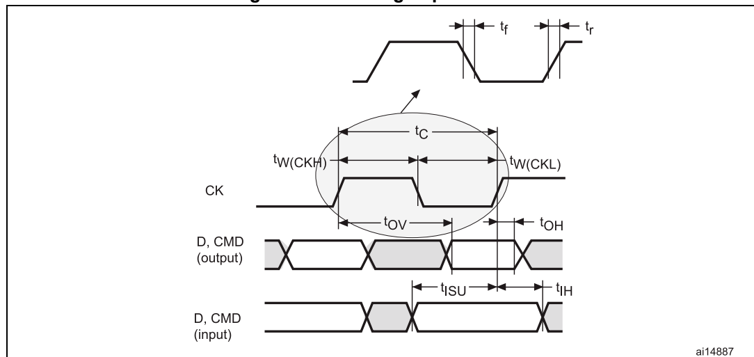
Figure 52. SDIO high-speed mode
