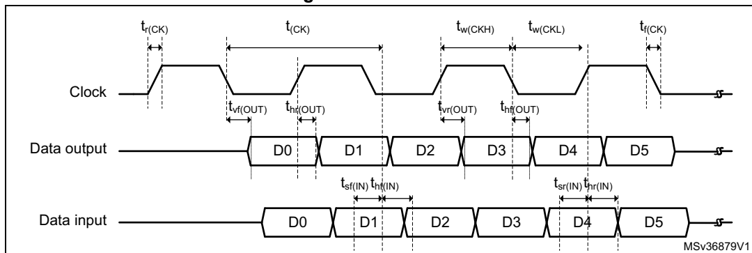
Figure 54. DDR mode
