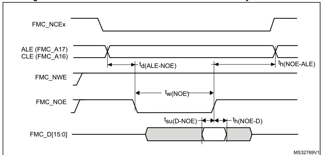
Figure 34. NAND controller waveforms for common memory write access
