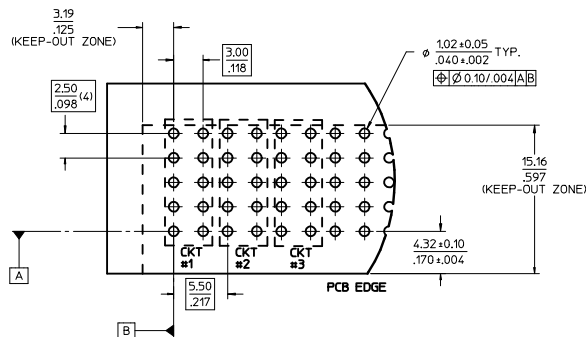
RECOMMENDED LAY-OUT AND KEEP-OUT ZONE SCALE 4:1
