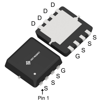
DFN3X3-8L (PowerFLAT-8(3.3x3.3))
