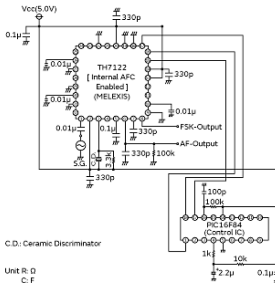
Measurement Circuit
